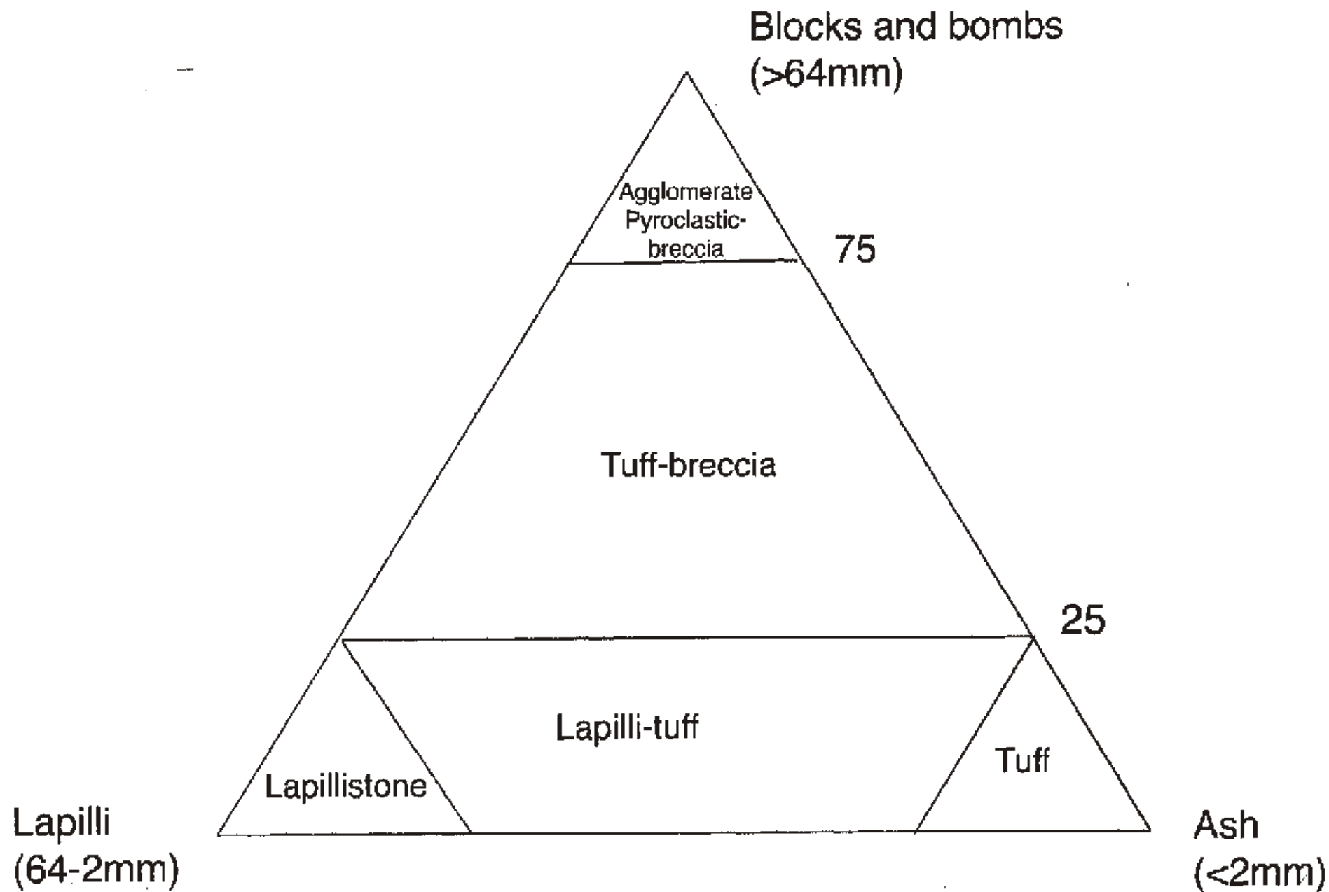
Classification of pyroclastic rocks
