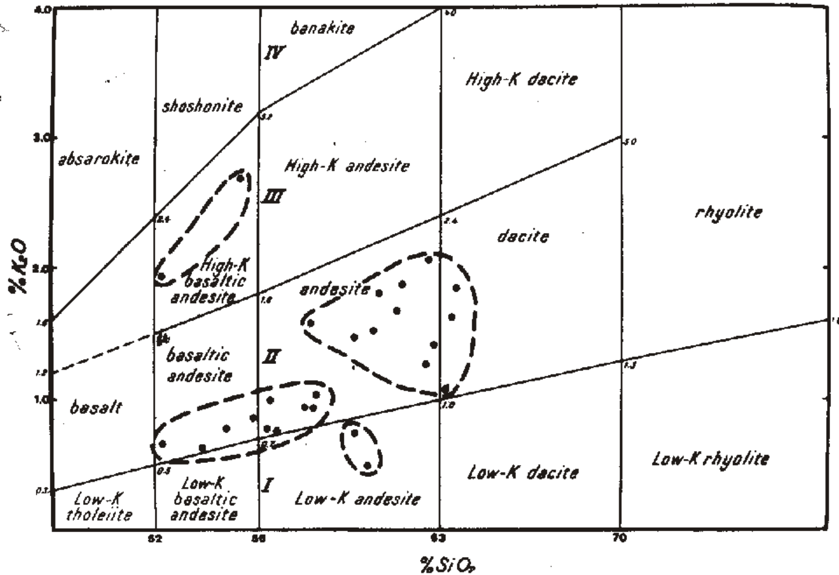
Fig. 2. Relationship between SiO 2 and K 2 O content. Lines on the K 2 O divisions mark the boundaries between: arc tholeiite series (I), calc-alkaline series (II), high-K calc-alkaline series (III) and shoshonite series (IV)
